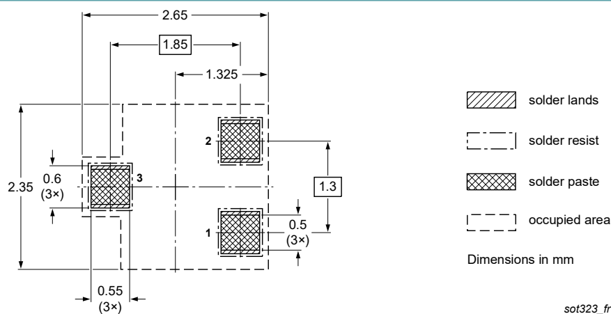
Fig. 7. Reflow soldering footprint for SC-70 (SOT323)
