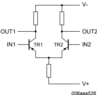
Fig. 10. Differential amplifier
