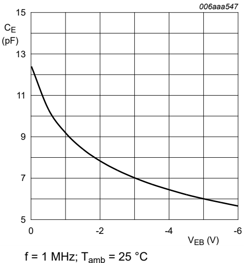
Fig. 8. Per transistor: Emitter capacitance as a function of emitter-base voltage; typical values
