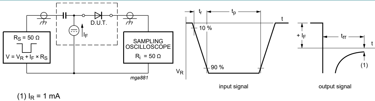
Fig. 13. Reverse recovery time: test circuit and waveforms
