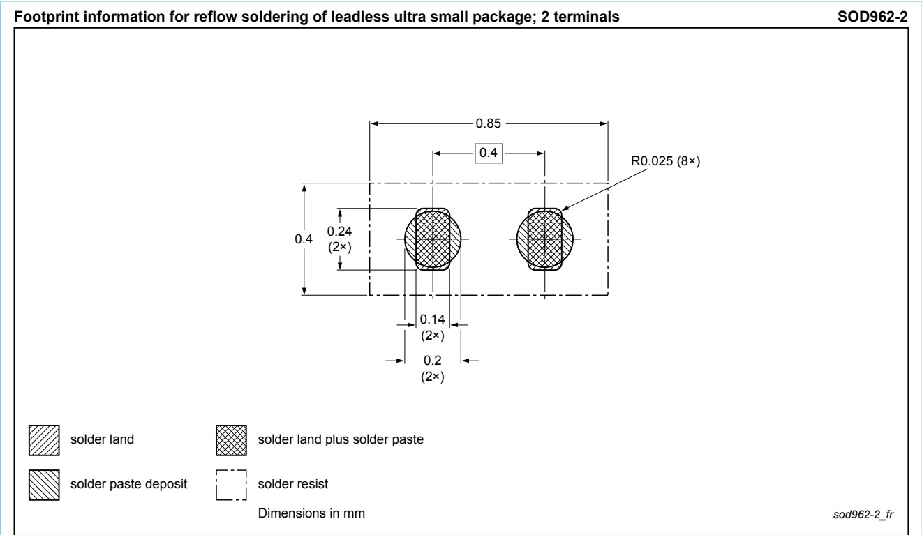
Fig. 16. Reflow soldering footprint for DSN0603-2 (SOD962-2)
