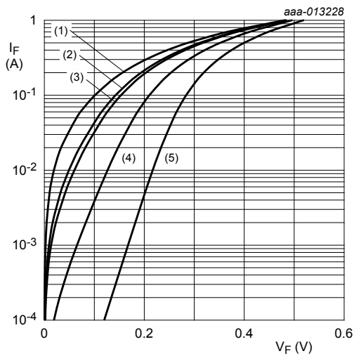
pulsed condition (1) T_j = 125^\circ\text{C} (2) T_j = 85^\circ\text{C} (3) T_j = 75^\circ\text{C} (4) T_j = 25^\circ\text{C} (5) T_j = -40^\circ\text{C}
