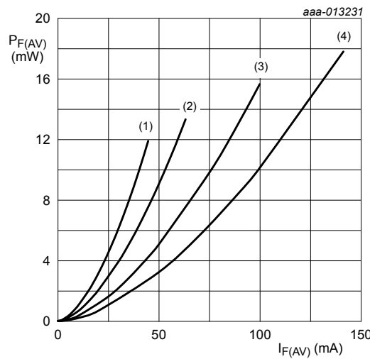
T_j = 125^\circ\text{C} (1) \delta = 0.1 (2) \delta = 0.2 (3) \delta = 0.5 (4) \delta = 1
