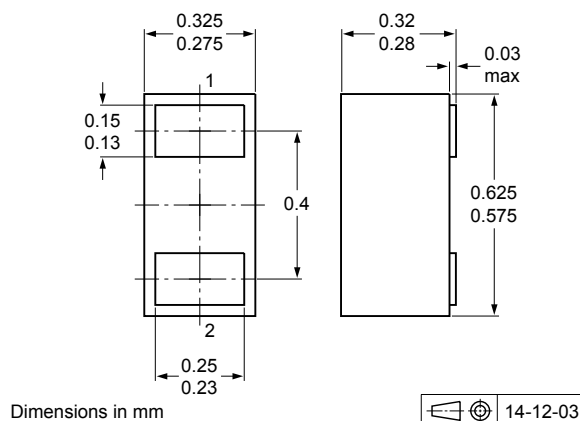
Fig. 15. Package outline DSN0603-2 (SOD962-2)
