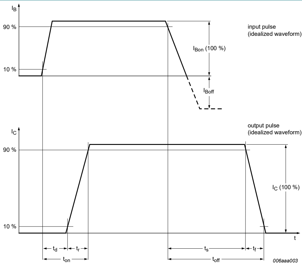
Fig. 12. Switching time definition
