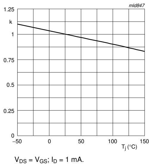
Fig 16. Temperature coefficient of gate-source threshold voltage as a function temperature; N-channel; typical values
