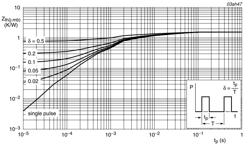
Fig 13. Transient thermal impedance from junction to mounting base as a function of pulse duration
