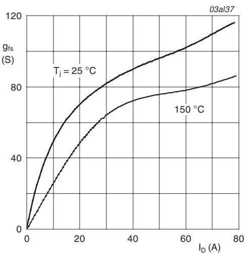
Fig 14. Forward transconductance as a function of drain current; typical values
