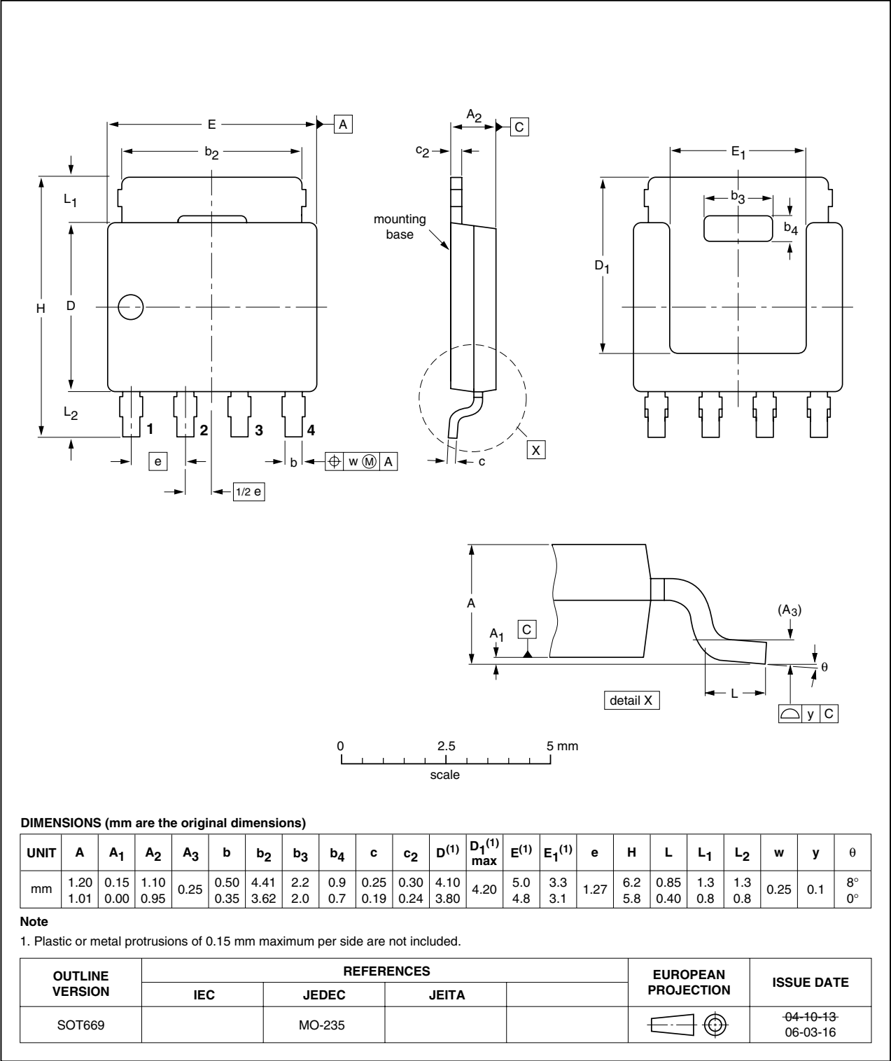
Fig 13. Package outline SOT669 (LPAK)
