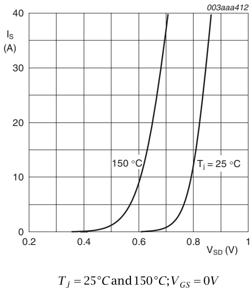
Fig 10. Source current as a function of source-drain voltage; typical values
