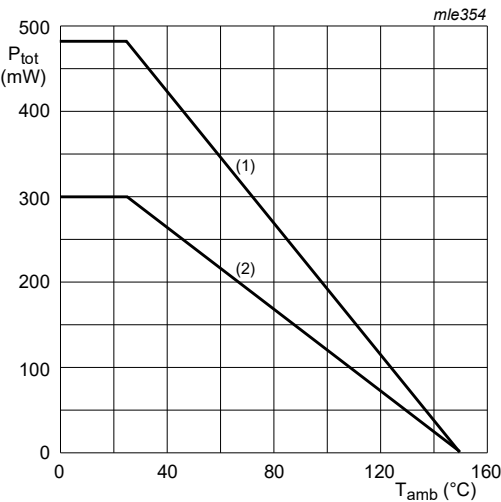
(1) FR4 PCB; 1 cm 2 copper mounting pad for collector. (2) Standard footprint.
