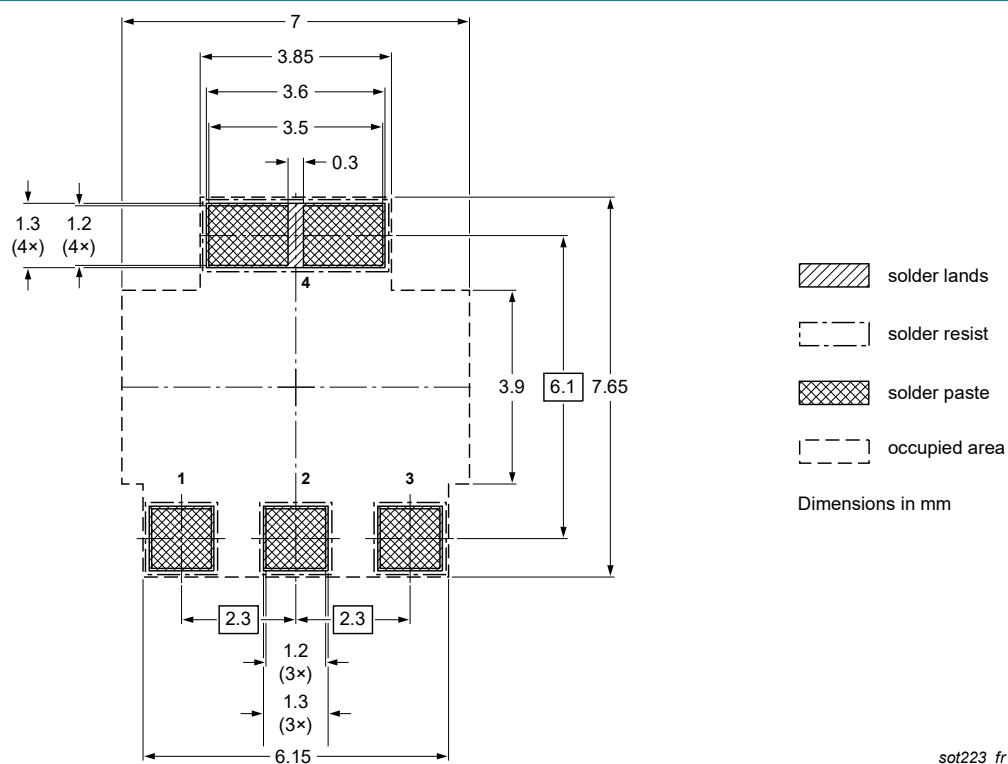
Fig. 9. Reflow soldering footprint for SC-73 (SOT223)
