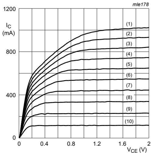
T_{amb} = 25^\circ\text{C} (1) I_B = 2600\ \mu\text{A} (2) I_B = 2340\ \mu\text{A} (3) I_B = 2080\ \mu\text{A} (4) I_B = 1820\ \mu\text{A} (5) I_B = 1560\ \mu\text{A} (6) I_B = 1300\ \mu\text{A} (7) I_B = 1040\ \mu\text{A} (8) I_B = 780\ \mu\text{A} (9) I_B = 520\ \mu\text{A} (10) I_B = 260\ \mu\text{A}
