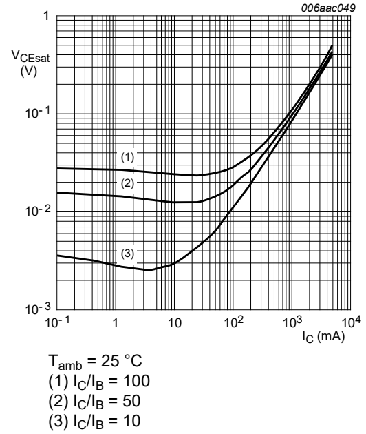
Fig. 13. Collector-emitter saturation voltage as a function of collector current; typical values
