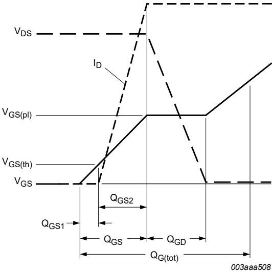
Fig. 15. Gate charge waveform definitions
