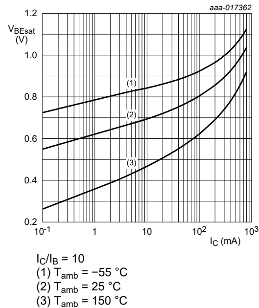
Fig. 5. NPN transistor: Base-emitter saturation voltage as a function of collector current; typical values
