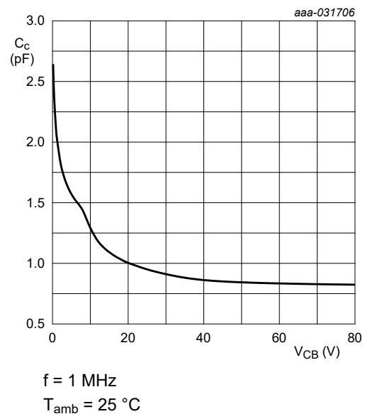
Fig. 14. NHUMH1: Collector capacitance as a function of collector-base voltage; typical values
