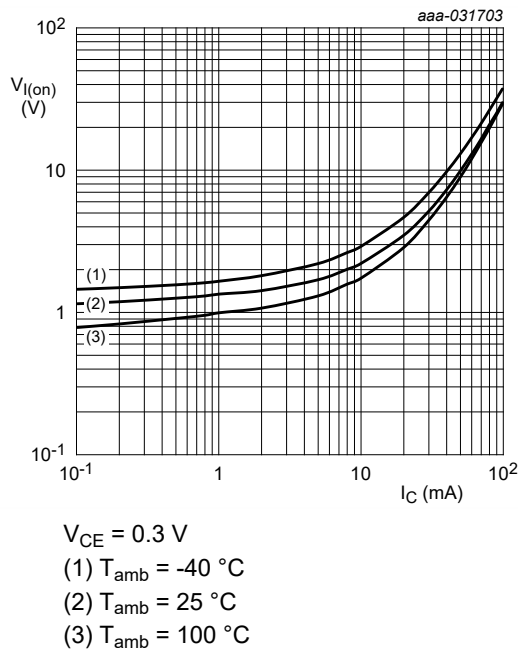
Fig. 12. NHDTC124EU: On-state input voltage as a function of collector current; typical values
