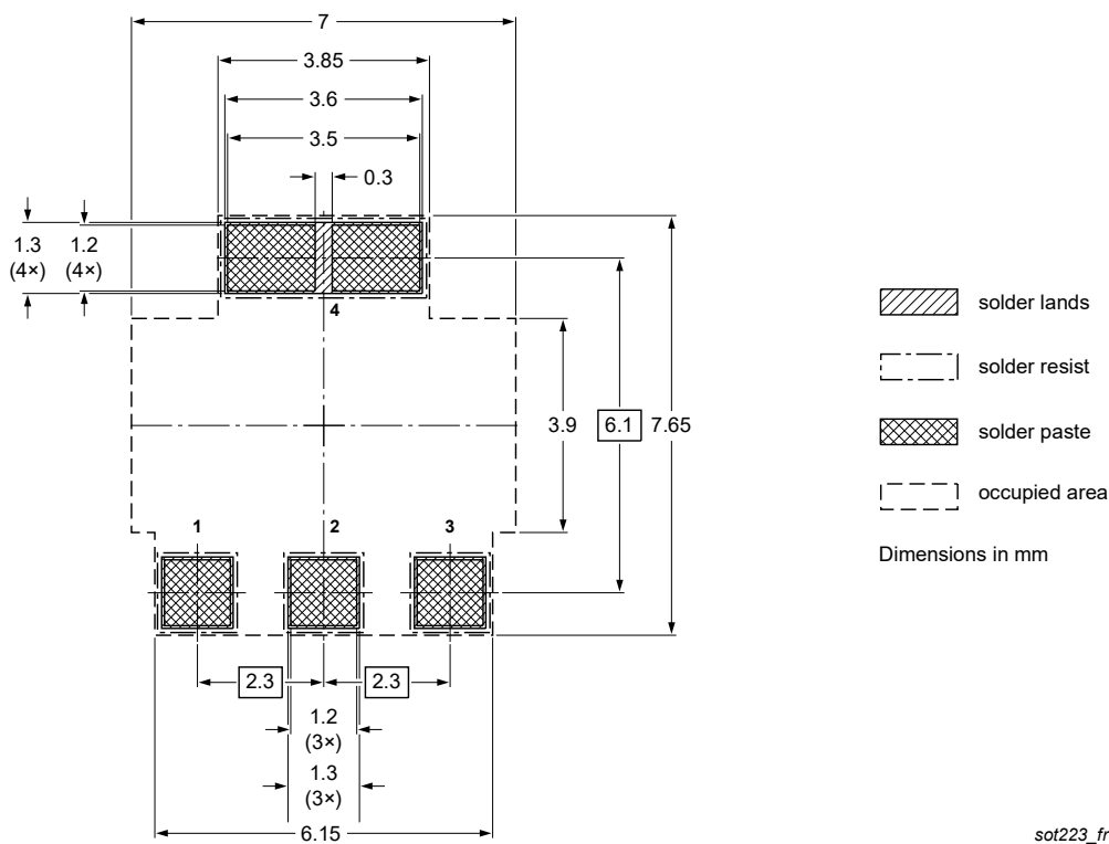
Fig. 5. Reflow soldering footprint for SC-73 (SOT223)
