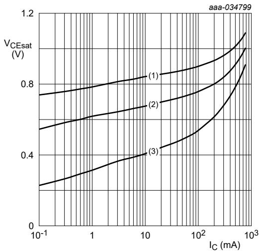
I_C/I_B = 1000 (1) T_{amb} = -55\text{ }^{\circ}\text{C} (2) T_{amb} = 25\text{ }^{\circ}\text{C} (3) T_{amb} = 150\text{ }^{\circ}\text{C}
