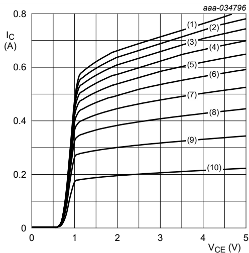
T_{amb} = 25\text{ }^{\circ}\text{C} (1) I_B = 35.0\text{ }\mu\text{A} (2) I_B = 31.5\text{ }\mu\text{A} (3) I_B = 28.0\text{ }\mu\text{A} (4) I_B = 24.5\text{ }\mu\text{A} (5) I_B = 21.0\text{ }\mu\text{A} (6) I_B = 17.5\text{ }\mu\text{A} (7) I_B = 14.0\text{ }\mu\text{A} (8) I_B = 10.5\text{ }\mu\text{A} (9) I_B = 7.0\text{ }\mu\text{A} (10) I_B = 3.5\text{ }\mu\text{A}
