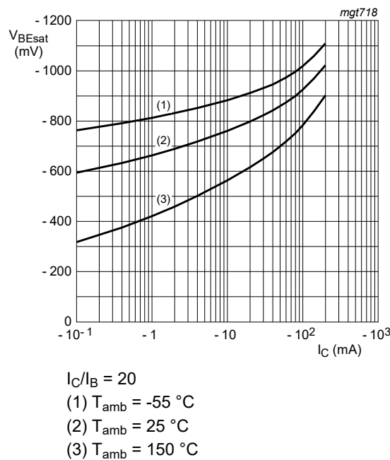
Fig. 9. BC856B-Q; BC857B-Q; BC858B-Q: Base-emitter saturation voltage as a function of collector current; typical values
