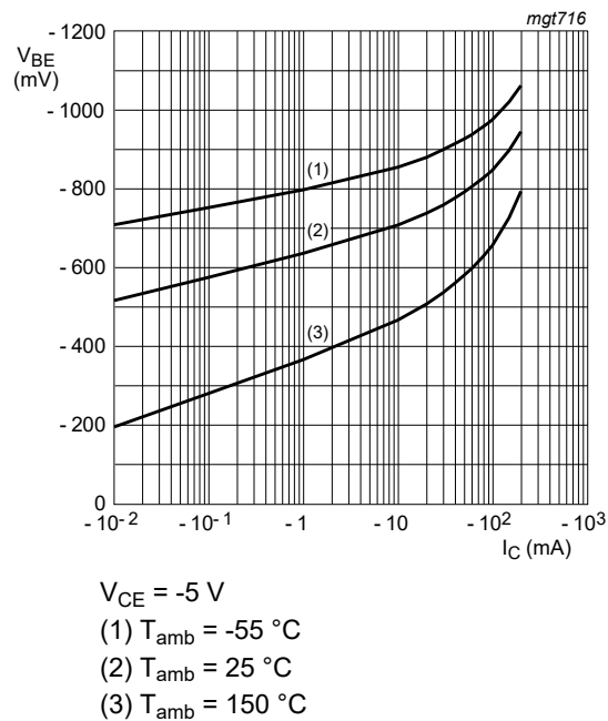
Fig. 7. BC856B-Q; BC857B-Q; BC858B-Q: Base-emitter voltage as a function of collector current; typical values
