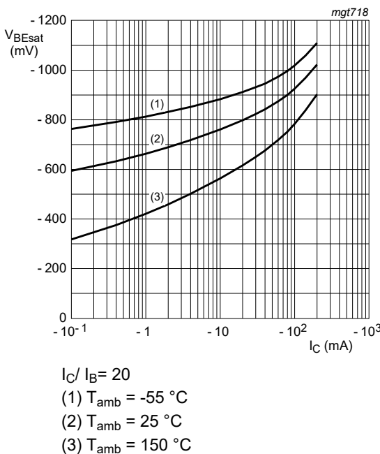
Fig. 11. BC857BQC-Q: Base-emitter saturation voltage as a function of collector current; typical values
