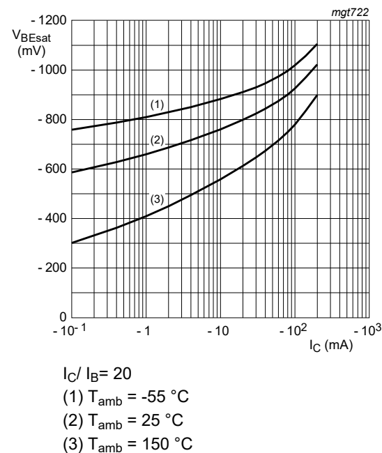
Fig. 15. BC857CQC-Q: Base-emitter saturation voltage as a function of collector current; typical values
