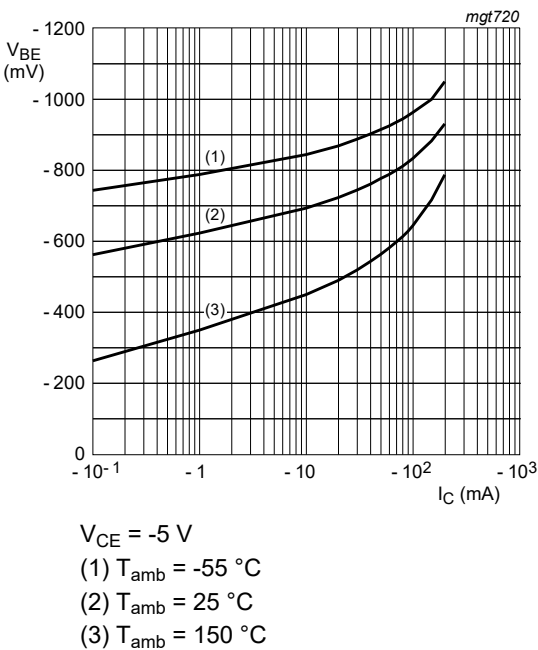
Fig. 11. BC857CW-Q: Base-emitter voltage as a function of collector current; typical values
