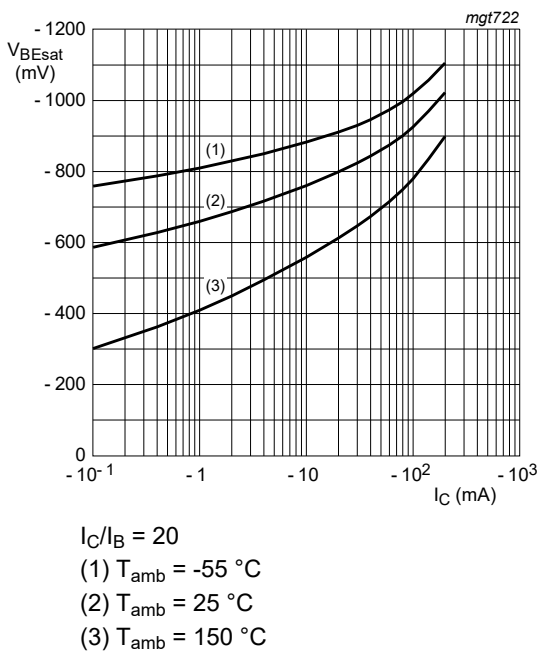
Fig. 13. BC857CW-Q: Base-emitter saturation voltage as a function of collector current; typical values
