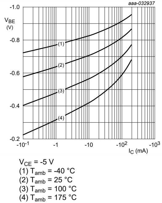
Fig. 4. Base-emitter voltage as a function of collector current; typical value
