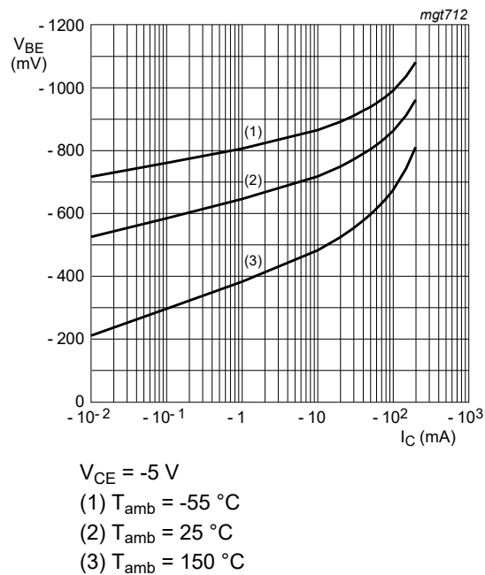
Fig. 5. BC856AQC-Q: Base-emitter voltage as a function of collector current; typical values
