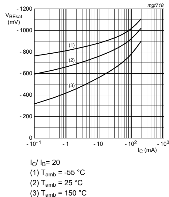
Fig. 11. BC856BQC-Q: Base-emitter saturation voltage as a function of collector current; typical values
