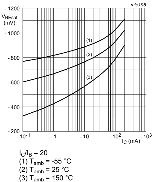
Fig. 13. PNP transistor: Base-emitter saturation voltage as a function of collector current; typical values
