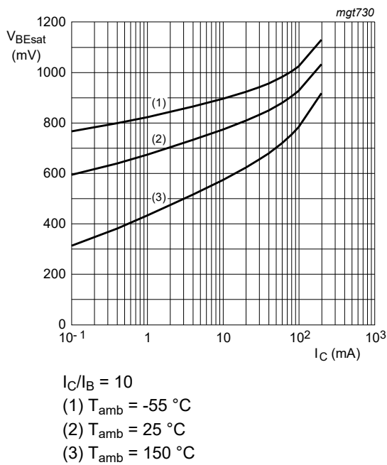
Fig. 9. BC847BW: Base-emitter saturation voltage as a function of collector current; typical values
