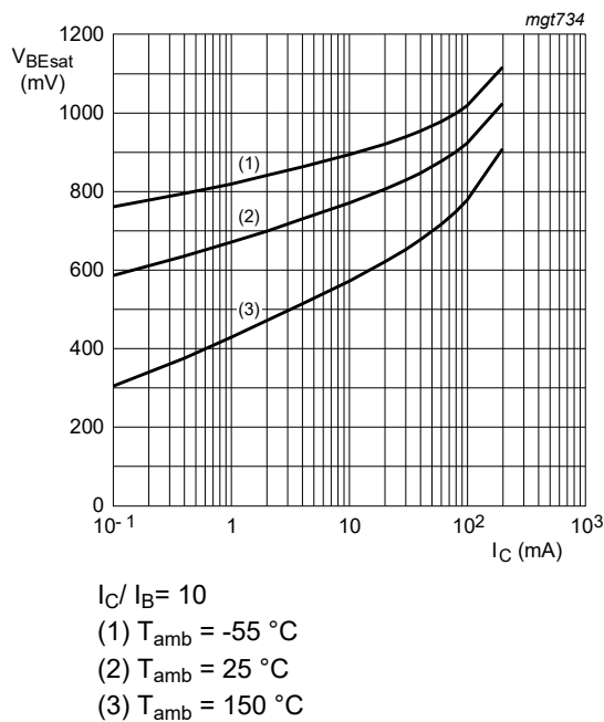
Fig. 15. BC847CQC-Q: Base-emitter saturation voltage as a function of collector current; typical values
