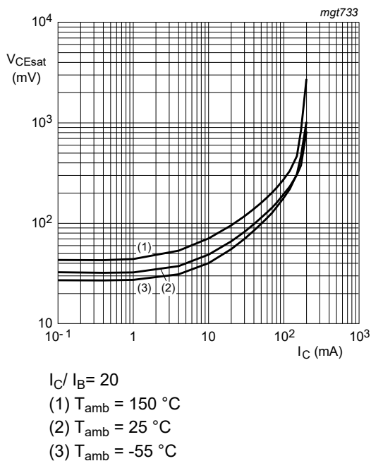
Fig. 14. BC847CQC-Q: Collector-emitter saturation voltage as a function of collector current; typical values
