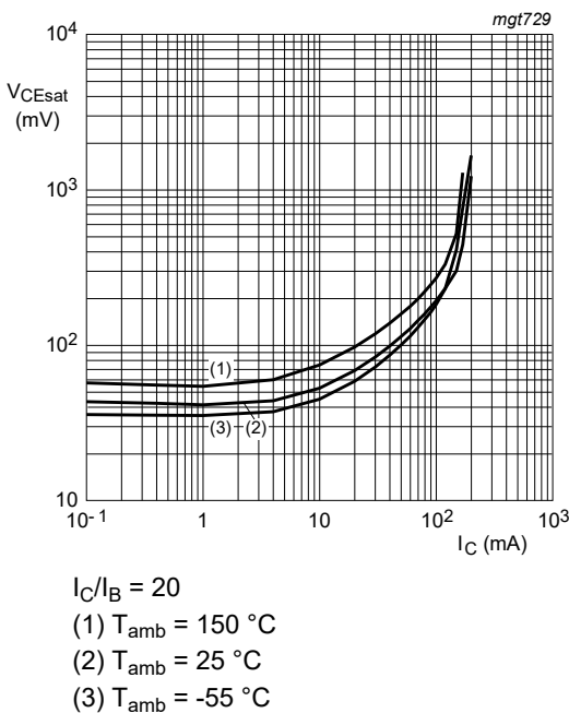
Fig. 8. BC847B-Q: Collector-emitter saturation voltage as a function of collector current; typical values
