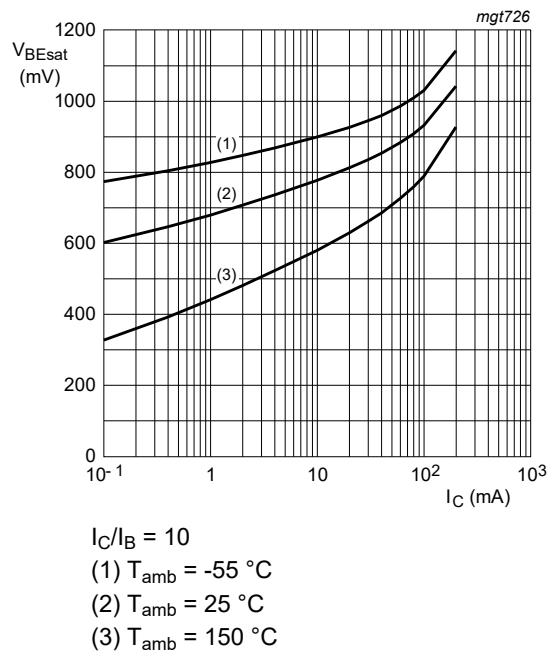
Fig. 5. BC847A-Q: Base-emitter saturation voltage as a function of collector current; typical values
