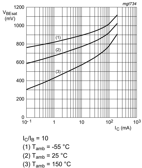
Fig. 13. BC847C-Q: Base-emitter saturation voltage as a function of collector current; typical values
