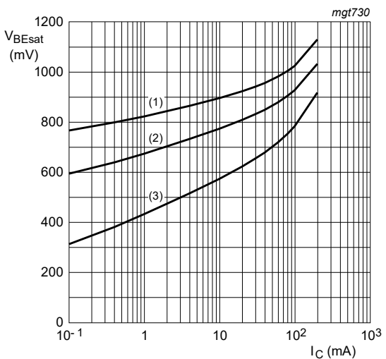
Fig. 9. BC847BQC-Q: Base-emitter voltage as a function of collector current; typical values
