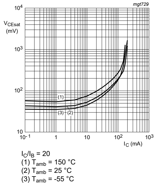
Fig. 8. TR1 (NPN): Collector-emitter saturation voltage as a function of collector current; typical values
