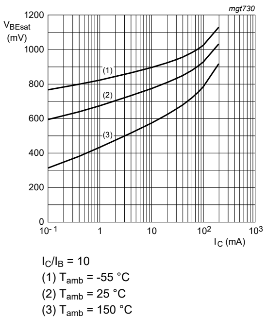
Fig. 9. BC847B-Q: Base-emitter saturation voltage as a function of collector current; typical values
