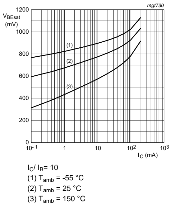
Fig. 11. BC847BQC: Base-emitter saturation voltage as a function of collector current; typical values
