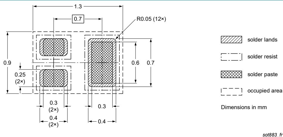
Fig. 15. Reflow soldering footprint SOT883 (SC-101)
