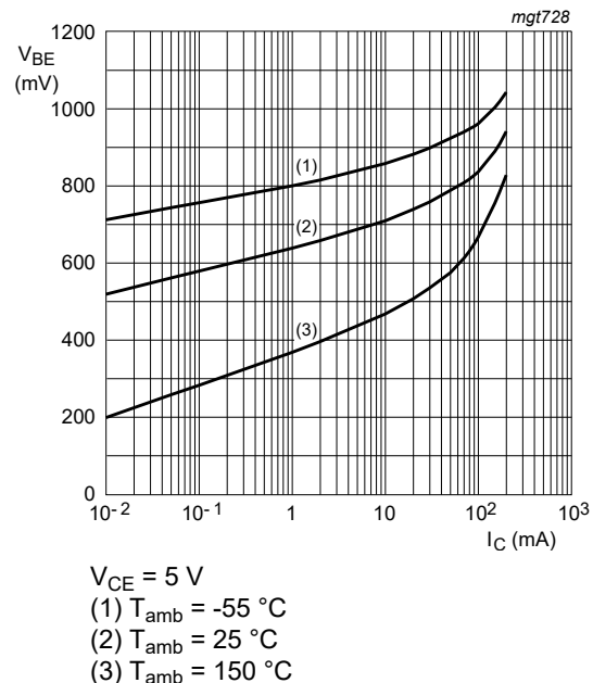
Fig. 5. Base-emitter voltage as a function of collector current; typical values
