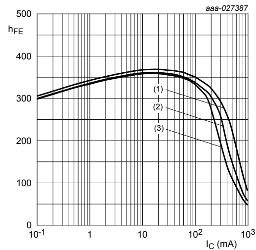
T_{amb} = 25 °C (1) V_{CE} = 5 V (2) V_{CE} = 2 V (3) V_{CE} = 1 V
