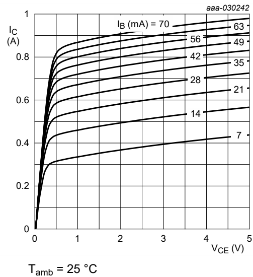
Fig. 5. BC816-16: Collector current as a function of collector-emitter voltage; typical values
