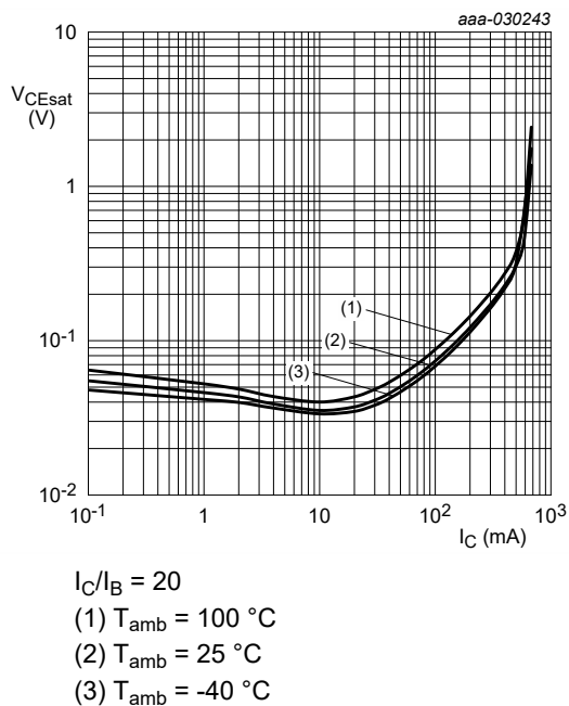
Fig. 6. BC816-16: Collector-emitter saturation voltage as a function of collector current; typical values
