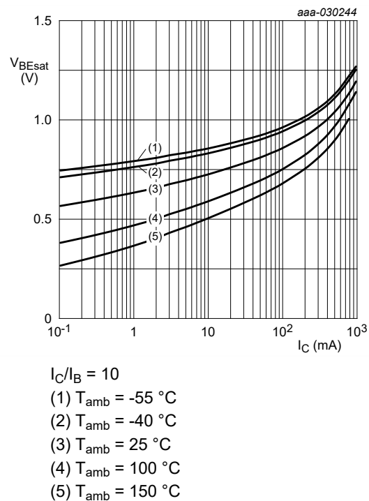
Fig. 7. BC816-16: Base-emitter saturation voltage as a function of collector current; typical values
