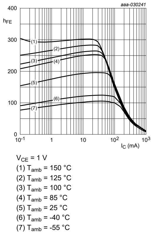
Fig. 4. BC816-16: DC current gain as a function of collector current; typical values
