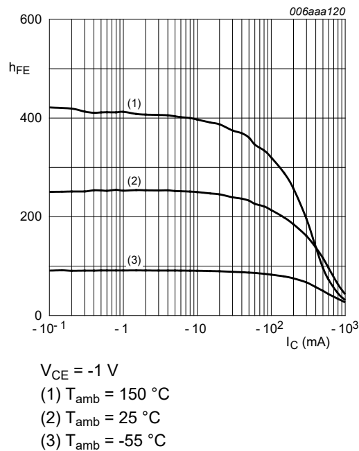
Fig. 8. BC807-25-Q: DC current gain as a function of collector current; typical values
