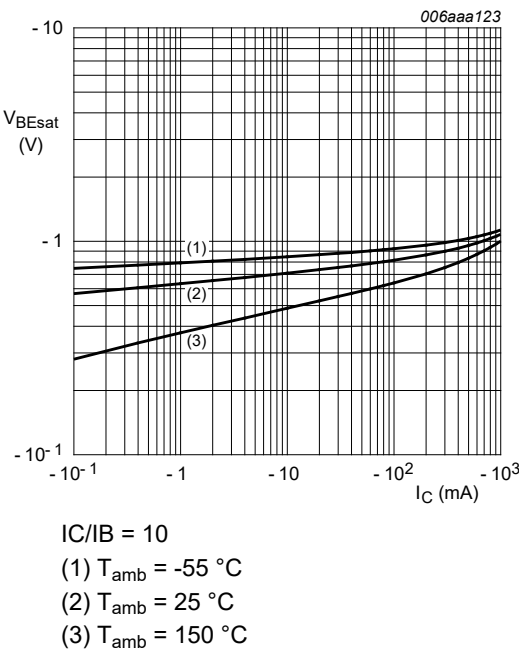
Fig. 9. BC807-25-Q: Base-emitter saturation voltage as a function of collector current; typical values
