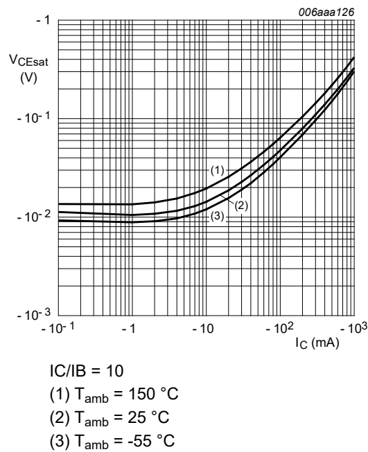
Fig. 10. BC807-25-Q: Collector-emitter saturation voltage as a function of collector current; typical values
