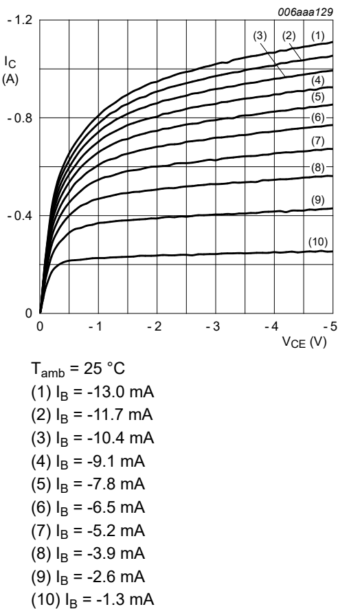
Fig. 11. BC807-25-Q: Collector current as a function of collector-emitter voltage; typical values
