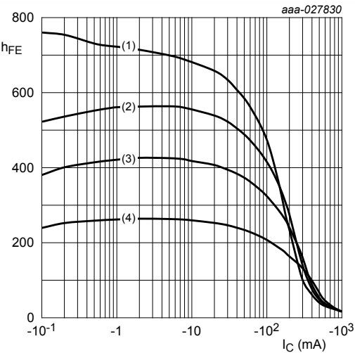
V_{CE} = -1\text{ V} (1) T_{amb} = 150\text{ °C} (2) T_{amb} = 85\text{ °C} (3) T_{amb} = 25\text{ °C} (4) T_{amb} = -40\text{ °C}
