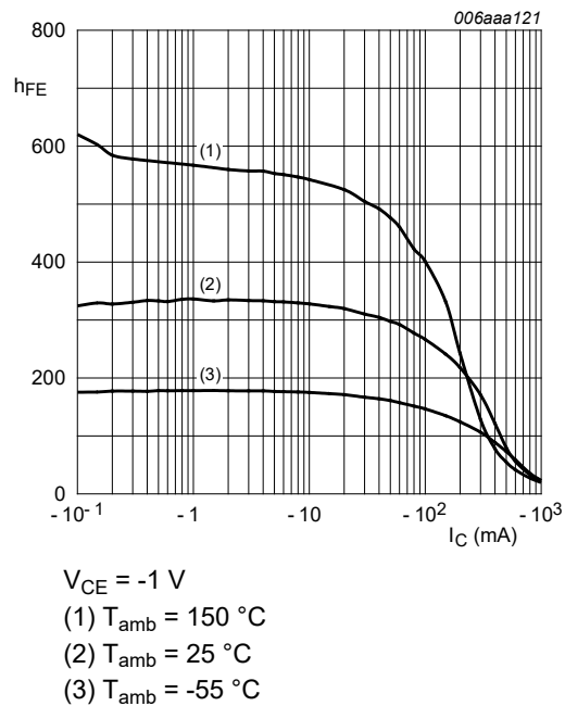
Fig. 12. BC807-40: DC current gain as a function of collector current; typical values
