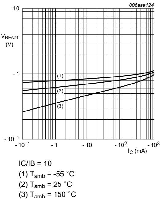
Fig. 13. BC807-40: Base-emitter saturation voltage as a function of collector current; typical values
