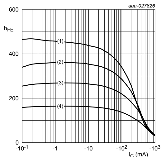
V_{CE} = -1\text{ V} (1) T_{amb} = 150\text{ °C} (2) T_{amb} = 85\text{ °C} (3) T_{amb} = 25\text{ °C} (4) T_{amb} = -40\text{ °C} Figure 6. BC807-25L, BC807-25LW: DC current gain as a function of collector current; typical values
