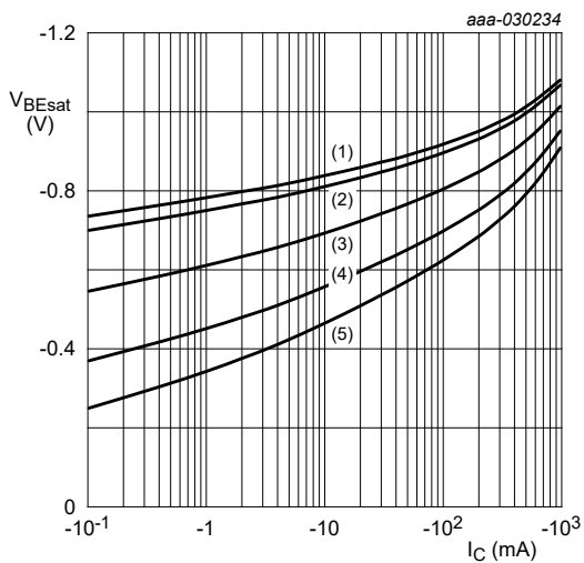
I_C/I_B = 10 (1) T_{amb} = -55\text{ }^{\circ}\text{C} (2) T_{amb} = -40\text{ }^{\circ}\text{C} (3) T_{amb} = 25\text{ }^{\circ}\text{C} (4) T_{amb} = 100\text{ }^{\circ}\text{C} (5) T_{amb} = 150\text{ }^{\circ}\text{C}
