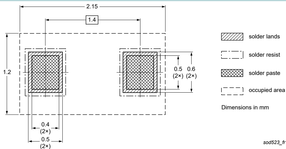
Fig. 5. Reflow soldering footprint for SC-79 (SOD523)
