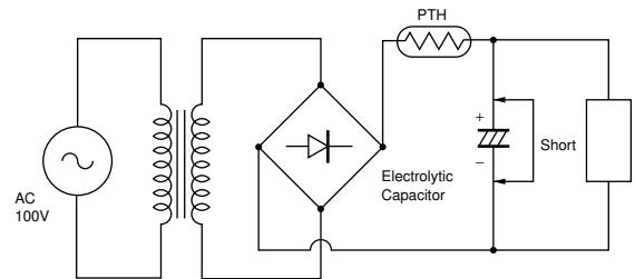
(4) Short-Circuit Test of Electrolytic Capacitor
