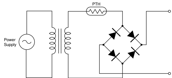
(3) Transformer Protection Circuit 2)
