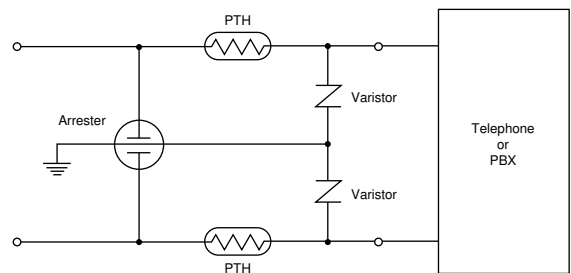
(5) Telecommunication Circuit
