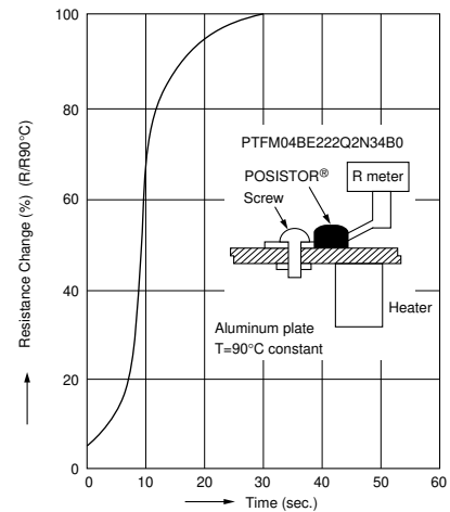
Operating Time of POSISTOR®
