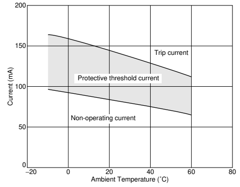
PTGL07AR750M7B52B0
