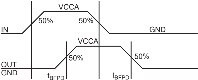
Figure 2-35. Buffer Module Waveform
