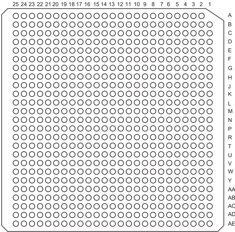
Figure 3-12. Package Bottom-View
