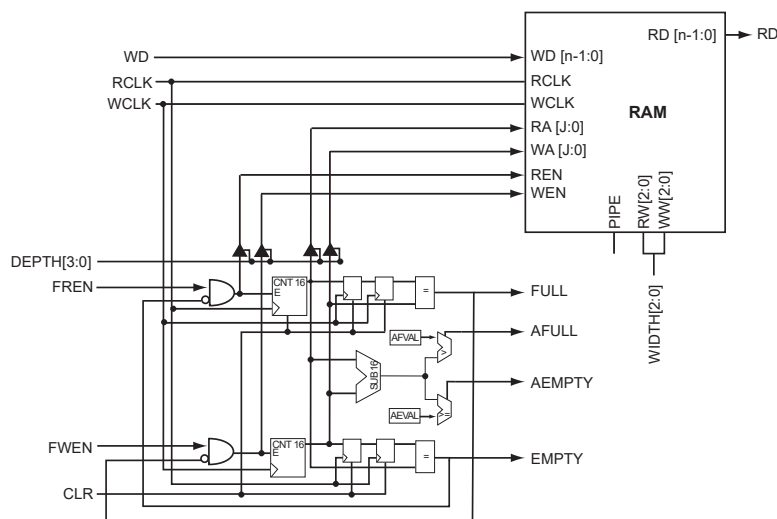
Figure 2-62. Axcelerator RAM with Embedded FIFO Controller
