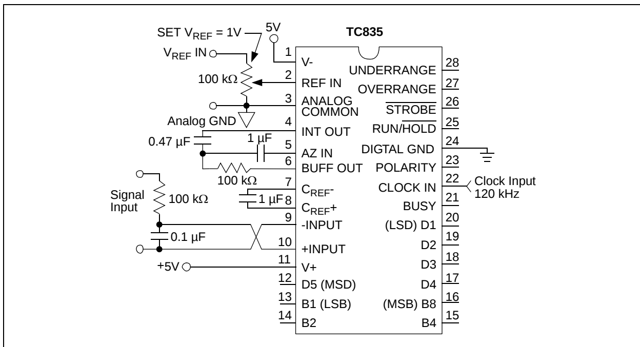
FIGURE 6-7: Test Circuit.
