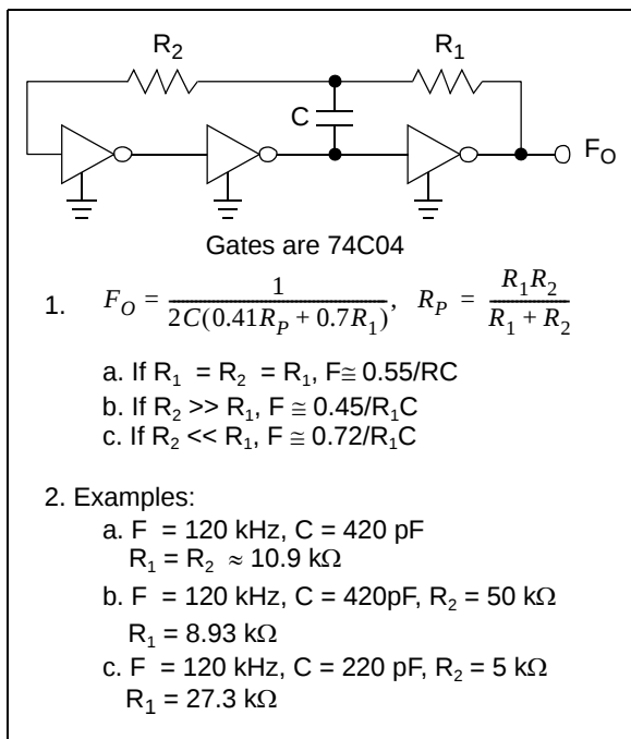
FIGURE 6-4: RC Oscillator Circuit.
