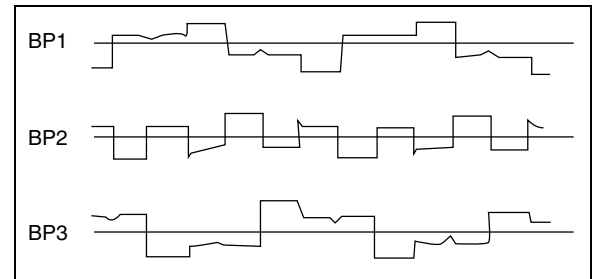
FIGURE 5-13: Backplane Waveforms.
