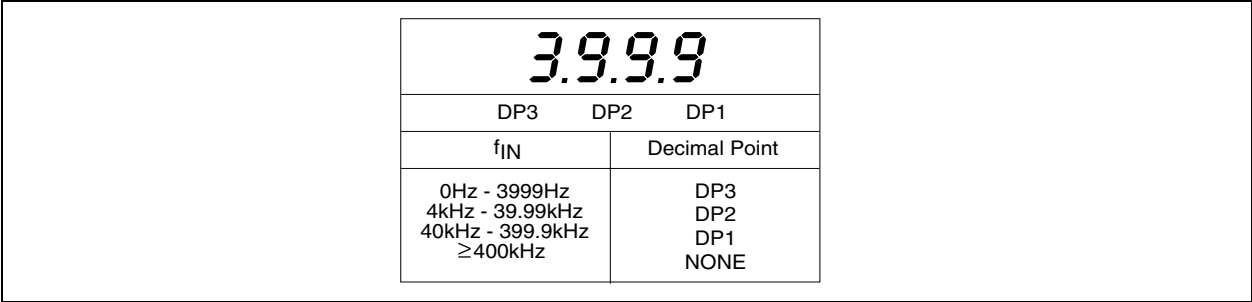
FIGURE 3-4: Auto-range Decimal Point Selection vs. Frequency Counter Input.
